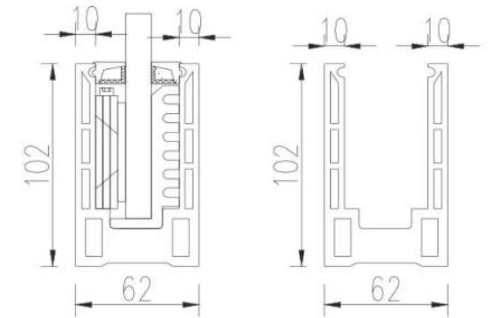
For 12mm to 15mm tempered glass
