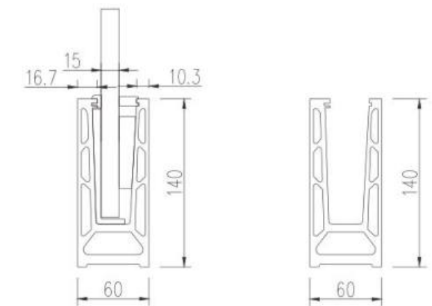
For 12mm to 19mm tempered glass
