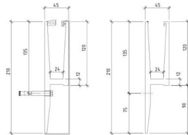
For 12mm to 6+1.52+6mm tempered laminated glass
