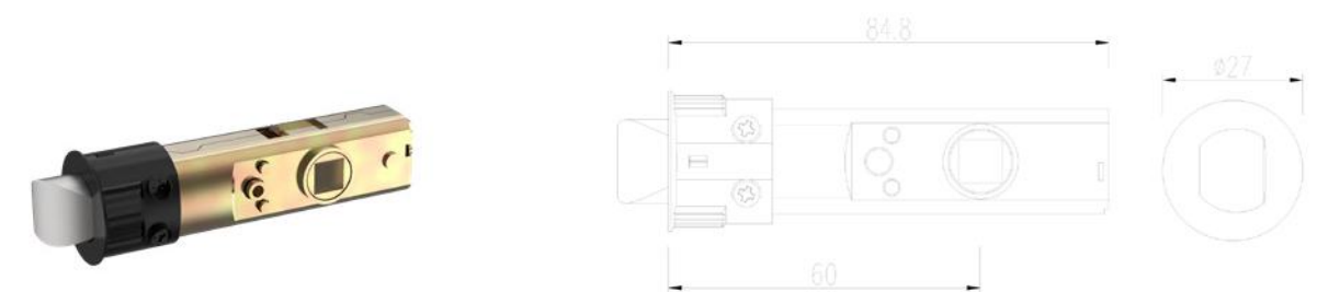
60 MM PRIVACY ROUND LATCH
