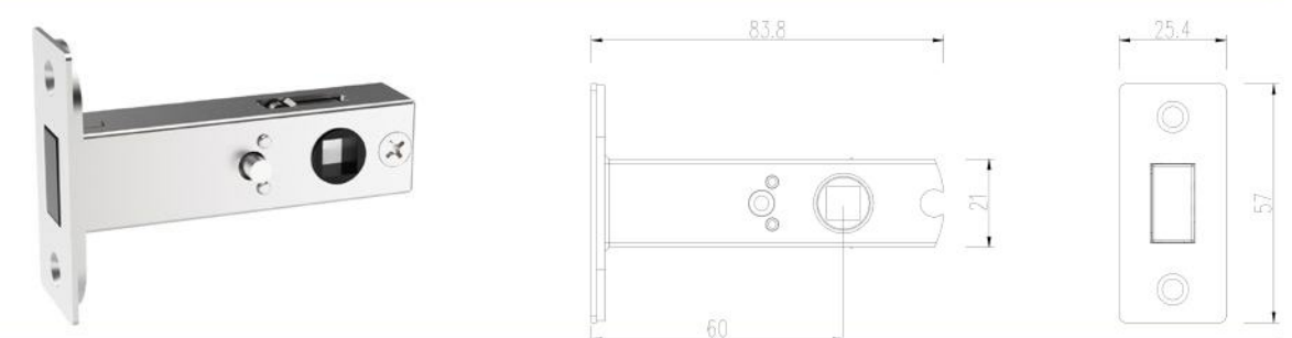
60 MAGNETIC PRIVACY LATCH
