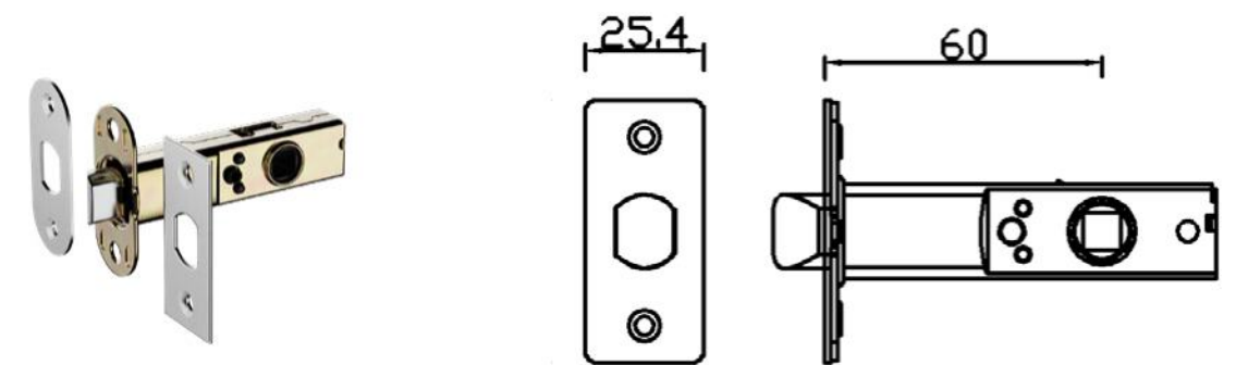
60MM PRIVACY LATCH
