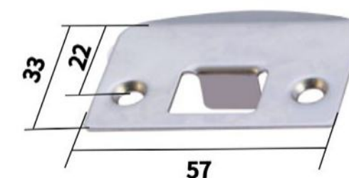
D-STRIKE PLATE
