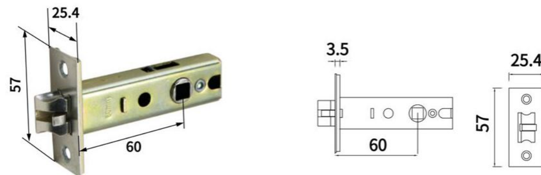
60MM TUBULAR LATCH
