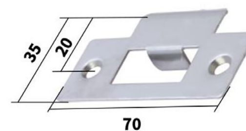
T-STRIKE PLATE
