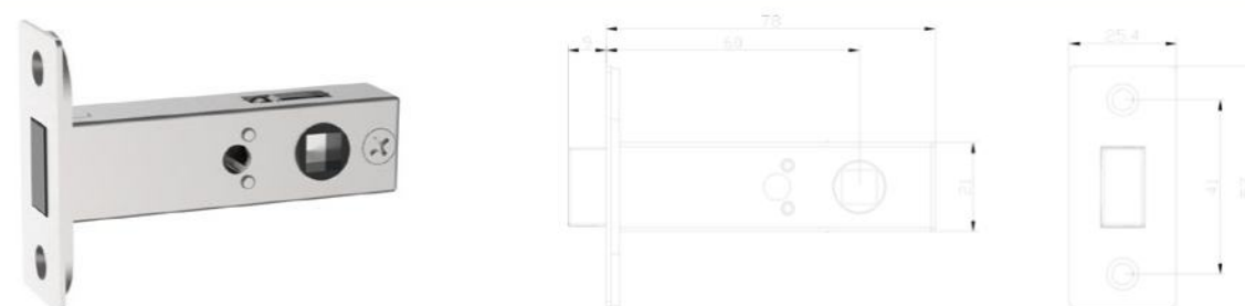
60 MM MAGNETIC LATCH
