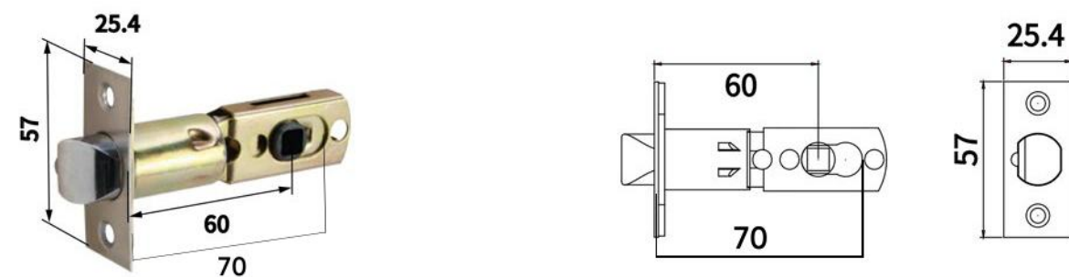
60-70MM ADJUSTABLE LATCH
