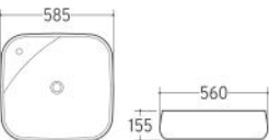
HY-8086 艺术盆 Art Basin Size: 585x560x155mm
