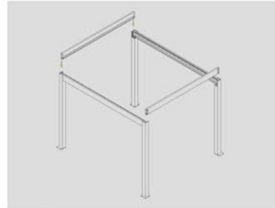
02 Assembly Frame
